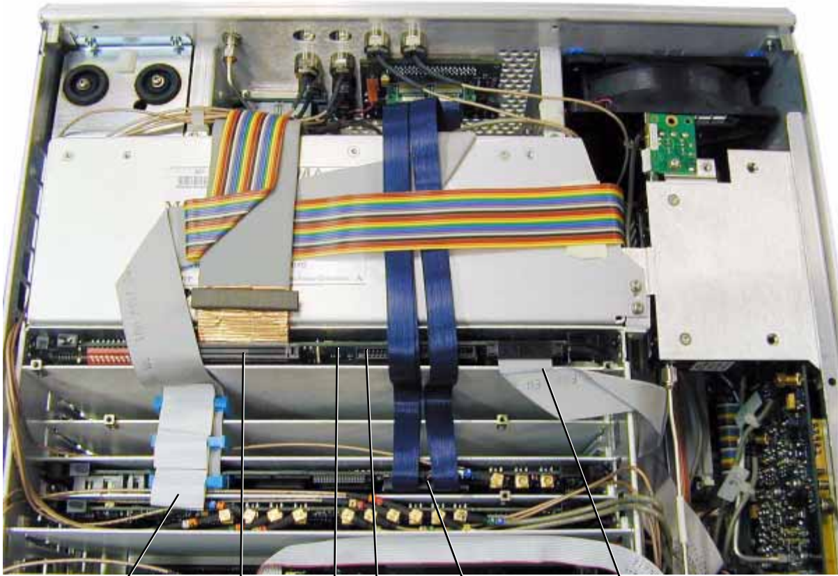
Figure 2-17 A18 CPU
