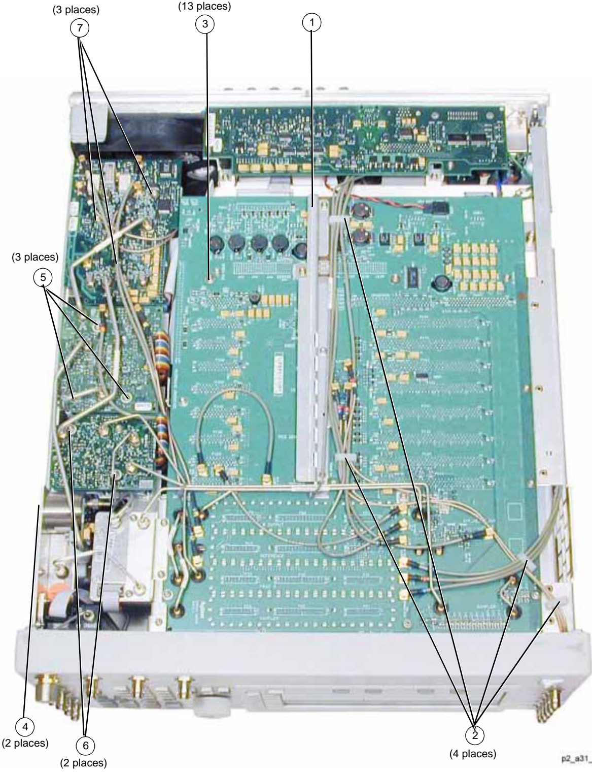
Figure 3-23 Main Chassis and MID Bottom View (E8267C)
