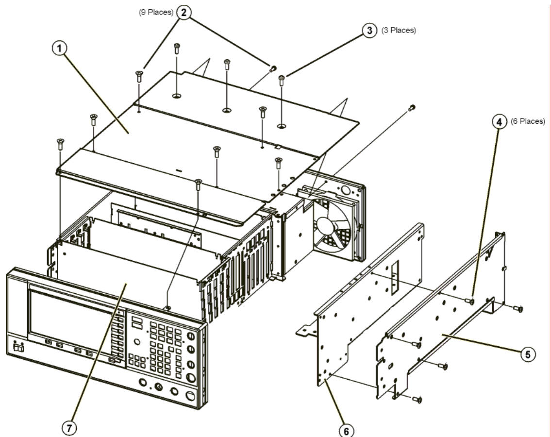
Figure 3-27 Main Chassis with Inside Cover and Right-Side Support Wall
